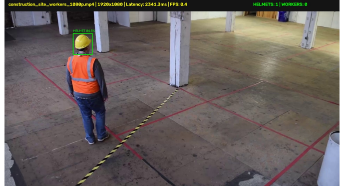
Fig. 1. Representative real-world construction surveillance scenario illustrating key challenges: distant tiny targets ( < 20 \times 20 px), heavy structural occlusions, variable illumination, and visual confusion between yellow safety helmets and background construction machinery/materials.
