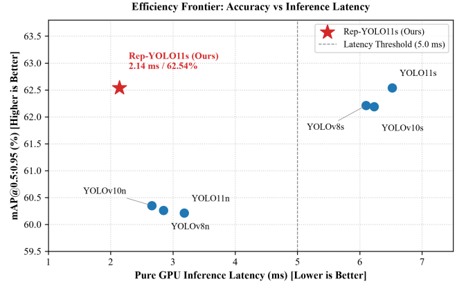
Fig. 3. Efficiency Frontier analysis displaying the trade-off between Pure GPU Inference Latency (ms) and mAP_{50-95} performance across tested model families.
