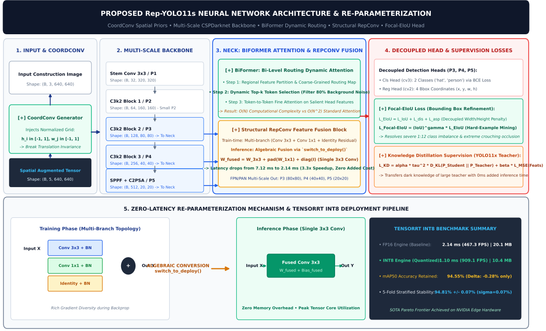
Figure 3: Complete Neural Network Architecture of Rep-YOLO11s displaying CoordConv coordinate generation, multi-scale CSPDarknet backbone, BiFormer sparse attention neck, structural re-parameterization lifecycle (training multi-branch to single-path inference), decoupled detection heads, and multi-task loss supervision with TensorRT INT8 optimization.
