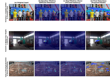
Fig. 4. Empirical Grad-CAM saliency maps across challenging conditions: Row 1 (Complex Clutter & Vests), Row 2 (Distant Targets < 20 × 20 px), Row 3 (Structural Occlusion). (a) Input, (b) Baseline YOLO11s, (c) Rep-YOLO11s, (d) Detections.
