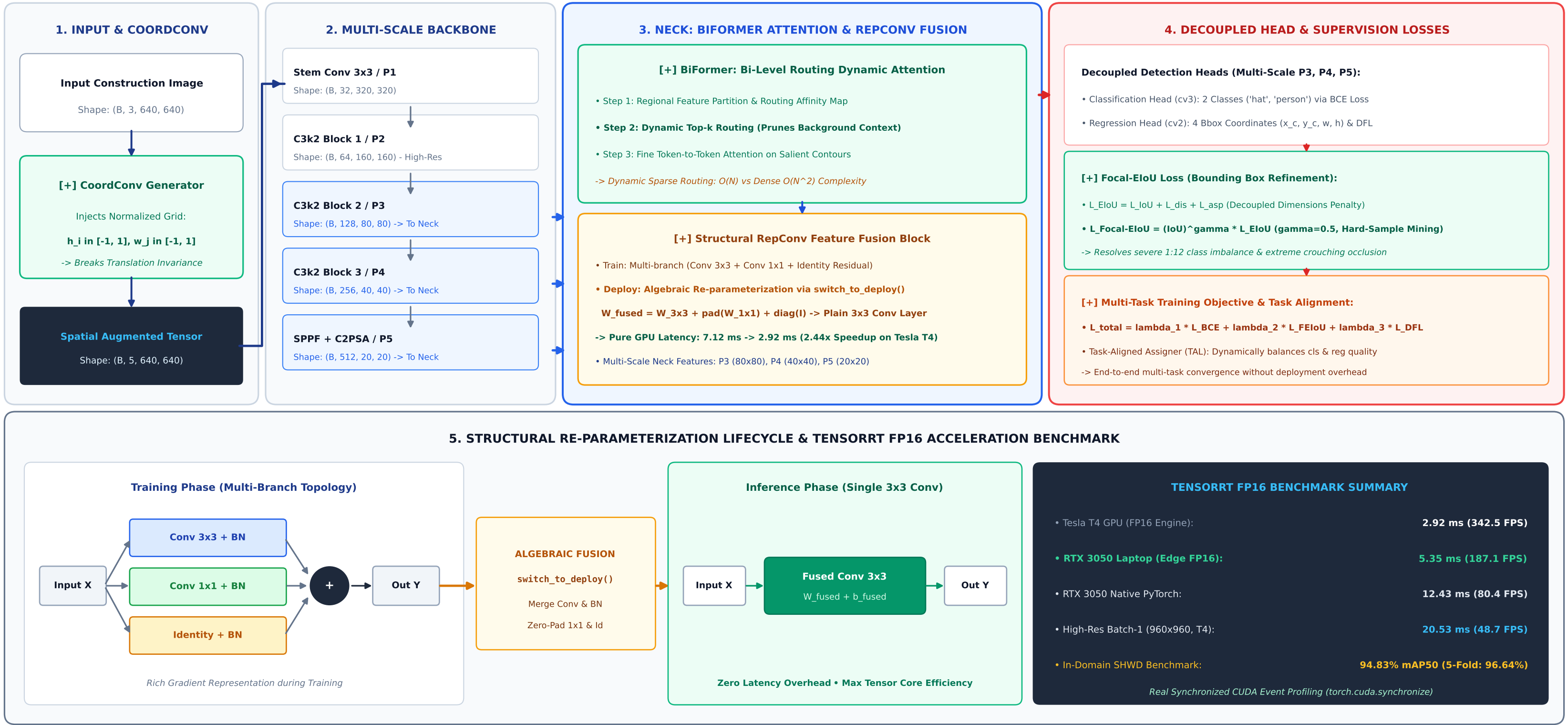
Figure 2: Complete Neural Network Architecture of Rep-YOLO11s displaying CoordConv coordinate generation, multi-scale CSPDarknet backbone, BiFormer sparse attention neck, structural re-parameterization lifecycle (training multi-branch to single-path inference), and decoupled heads with TensorRT FP16 acceleration.
