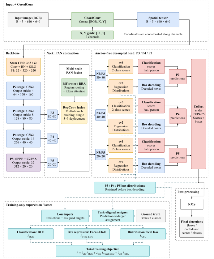
Fig. 1. Overall Architecture of Rep-YOLO11s. The pipeline integrates: (1) Stem CoordConv ( [RGB, X, Y] \rightarrow 5 \times 640 \times 640 ); (2) Multi-scale backbone (P1 Stem, P2–P4 C3k2, P5 SPFP+C2PSA); (3) PAN neck with Bi-Level Routing Attention (BRA) and RepConv; (4) Decoupled detection heads (cv3, cv2); and (5) Decoupled multi-task loss supervision with TAL, Focal-EIoU, and DFL.
