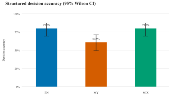
Fig. 2. Fig. 2. Structured decision accuracy with 95% Wilson intervals. Accuracy concerns the ANSWER/ABSTAIN decision, not semantic answer correctness.
