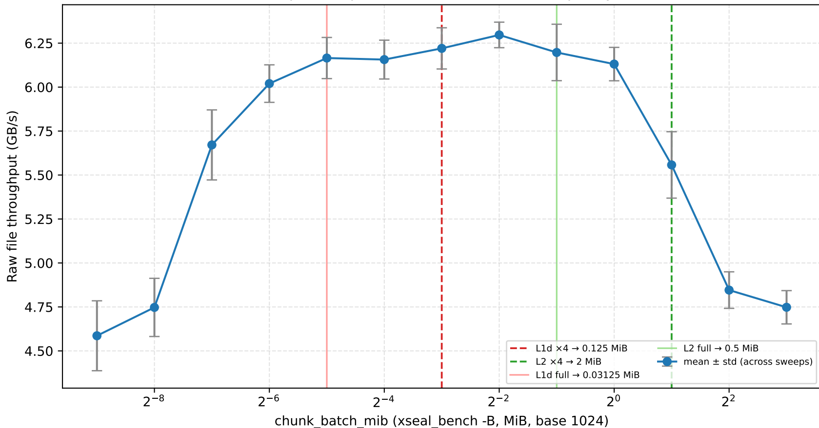
Chunk sweep (mmap); L1d/L2 full (solid), \times 4 capacity (dashed)
