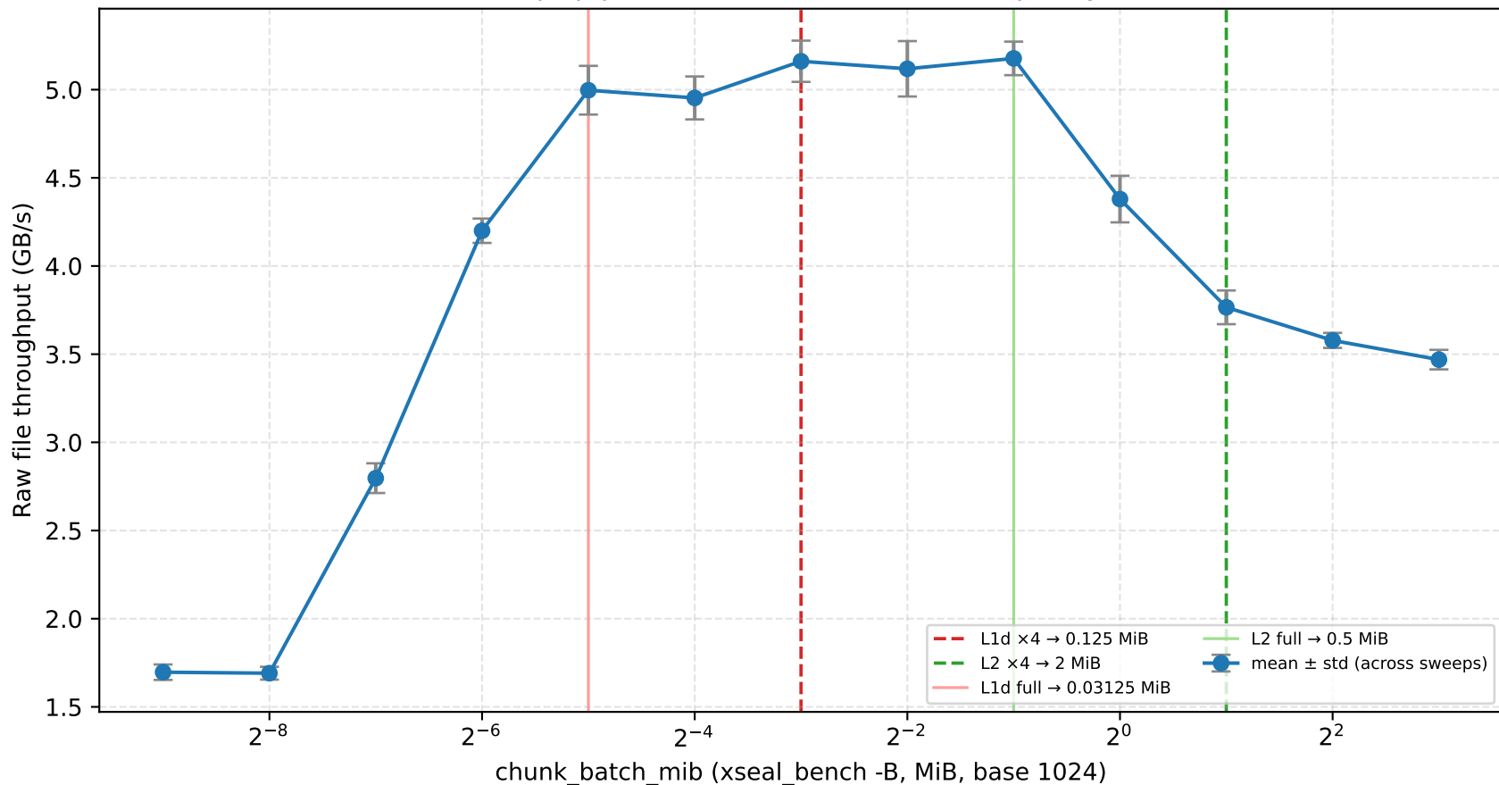
Chunk sweep (pipe); L1d/L2 full (solid), \times 4 capacity (dashed)
