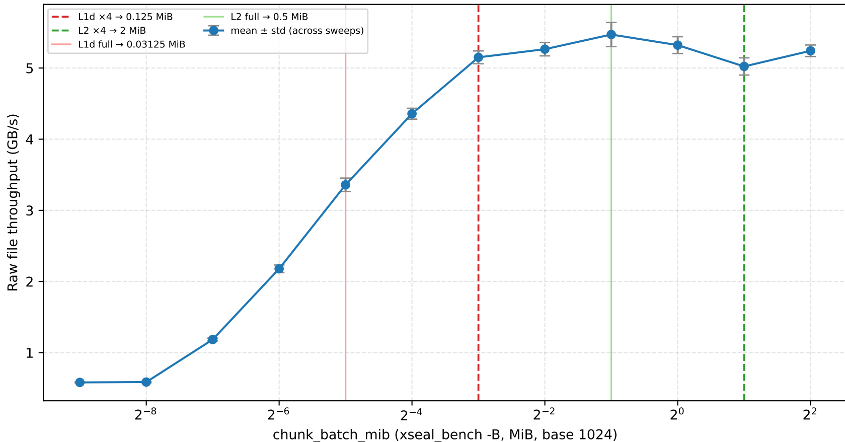
Chunk sweep (uring); L1d/L2 full (solid), \times 4 capacity (dashed)
