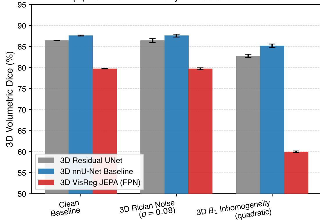
(A) Volumetric Accuracy Across Scanner Shifts
