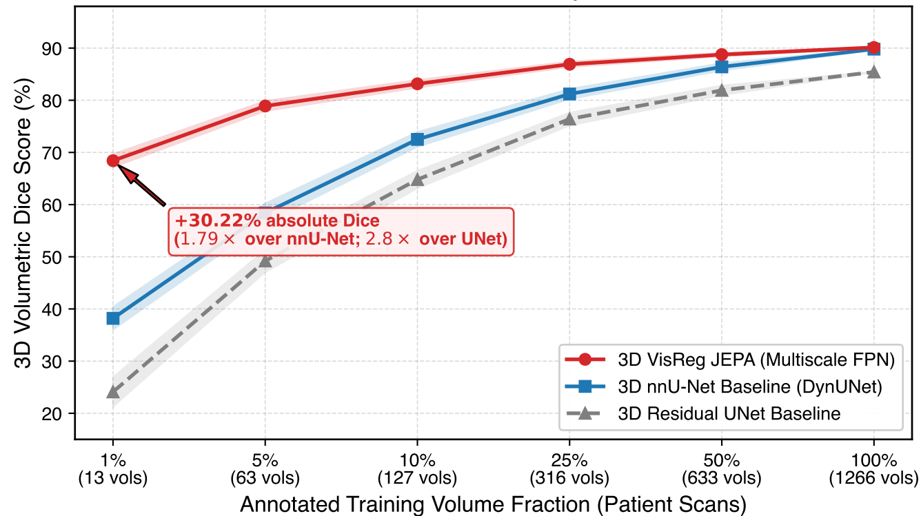
Low-Data Volumetric Label Efficiency on BraTS 2024 GLI
