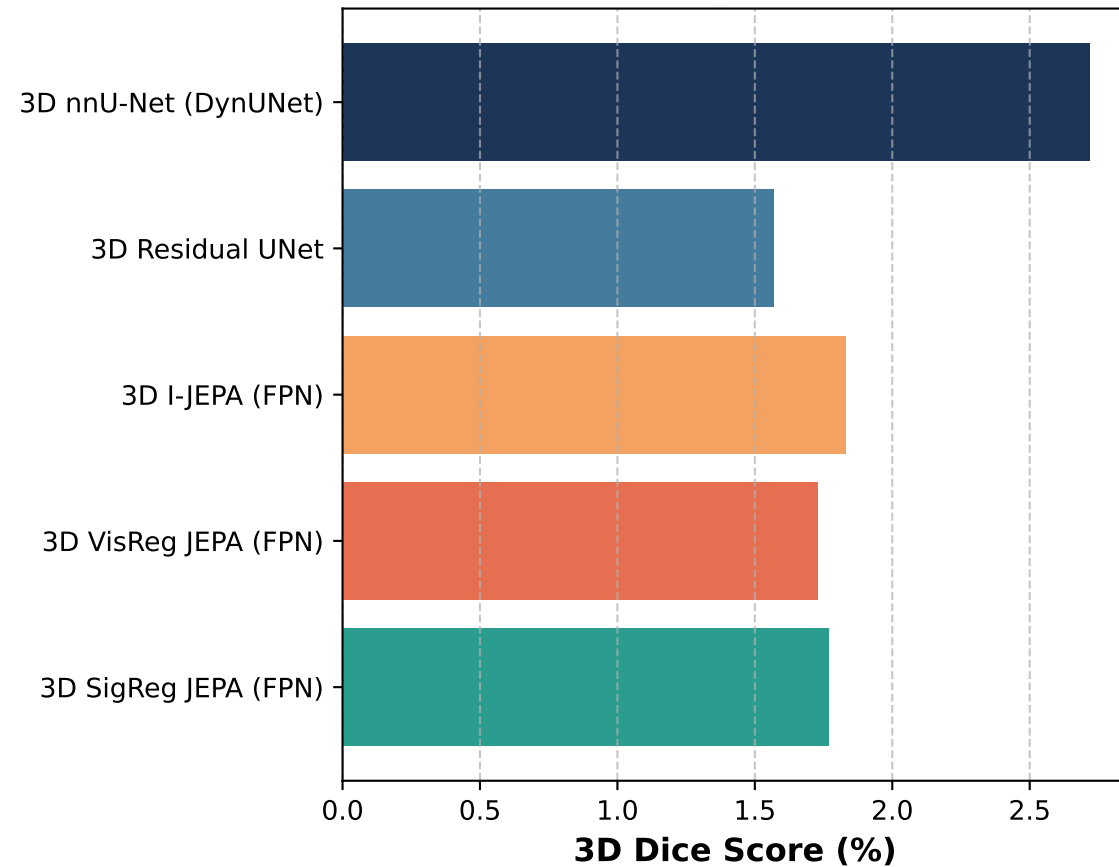
Volumetric Segmentation Dice
