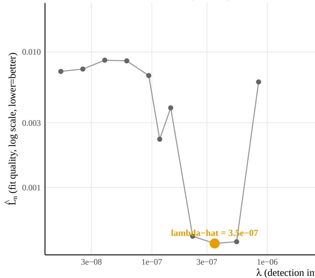
Instrument 1 ( m^*[t-1] )
