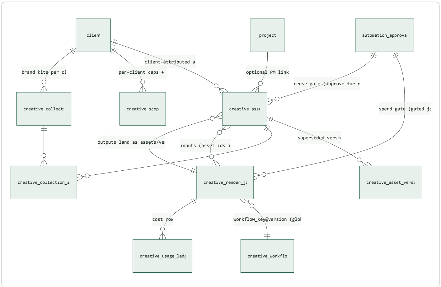
FIG. 04-1 – Entity map. creative_render_jobs is the state-machine spine; creative_workflows is the single global source of license truth every job resolves against.
