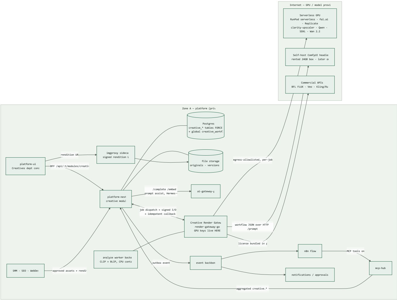
FIG. 02-1 – Master system diagram. Bytes flow storage → gateway → backend → gateway → storage via short-lived signed URLs platform-nest issues per job; the gateway persists nothing tenant-owned. imgproxy is a stateless sidecar reading the same storage, serving signed, on-the-fly renditions to the UI and to consuming departments.
