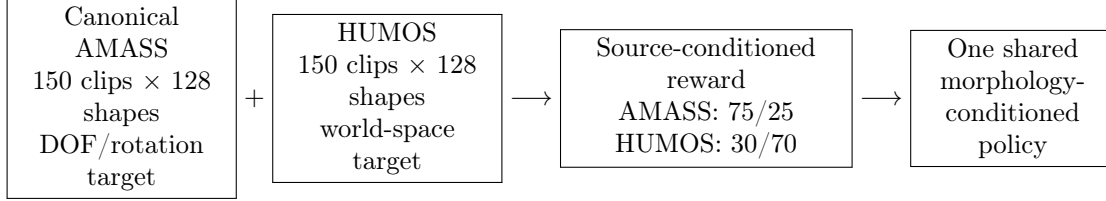
Figure 1: Current source-weighted training pipeline. AMASS/HUMOS episodes are sampled 50/50; both receive all tracking factors with source-specific DOF/world weights.
