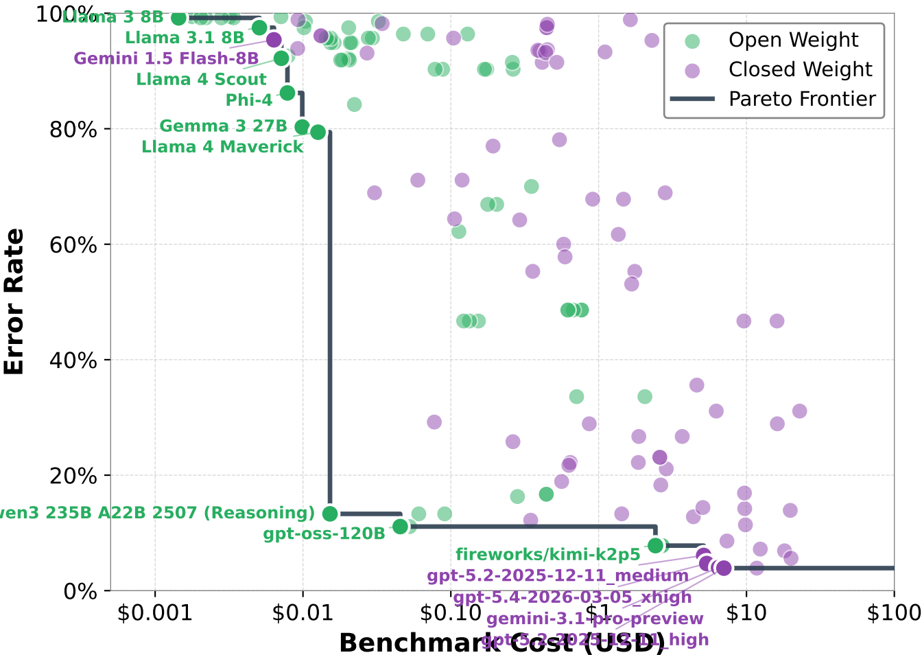
AIME Pareto Frontier with Model Names
