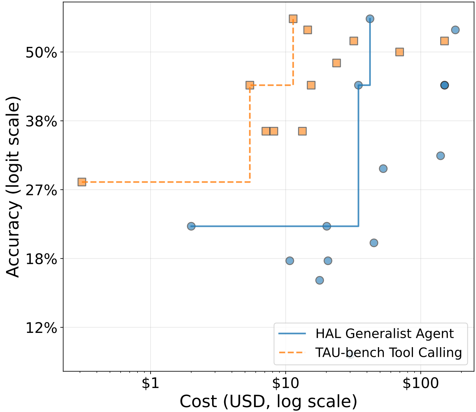
SciAgentBench
