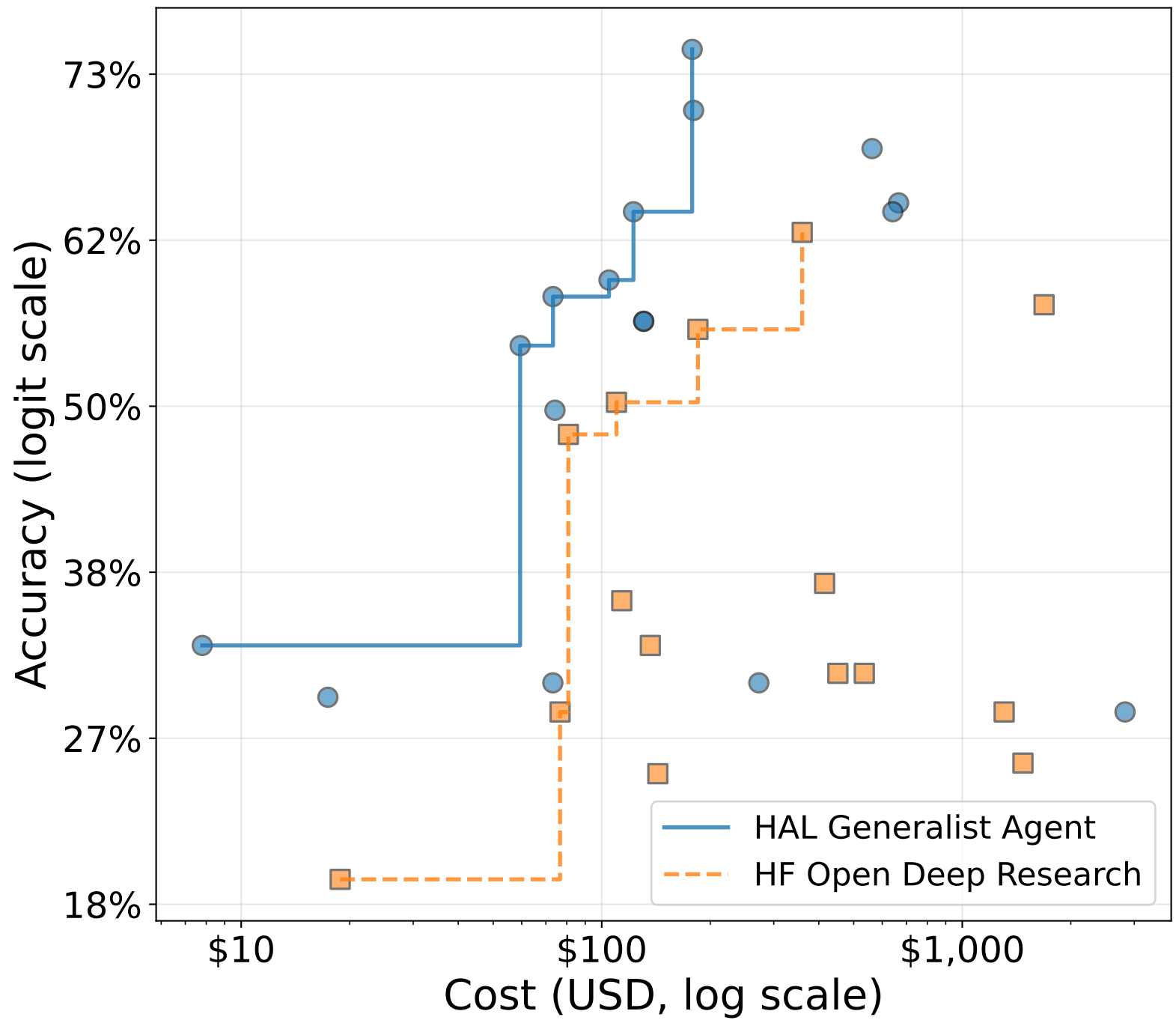
TAU-bench Airline
