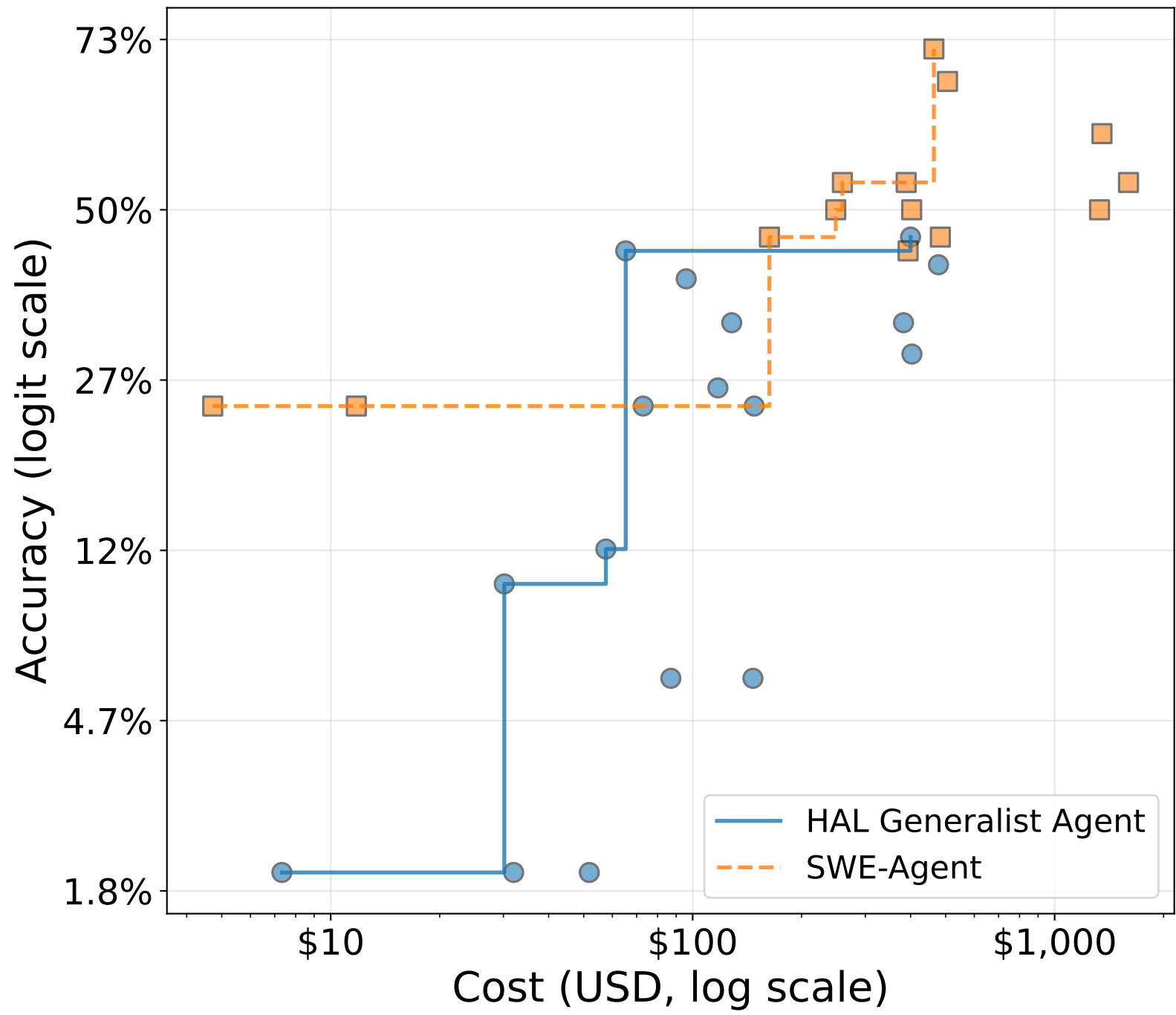
CORE-bench Hard
