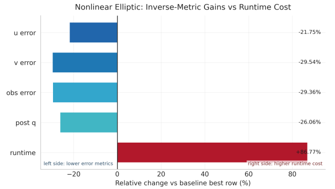
Figure 2: Relative changes versus baseline for best inverse row. Error metrics decrease while runtime increases, quantifying the gain-cost tradeoff directly.
