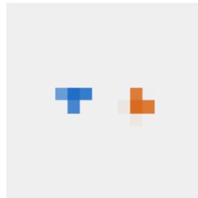
Balanced training
