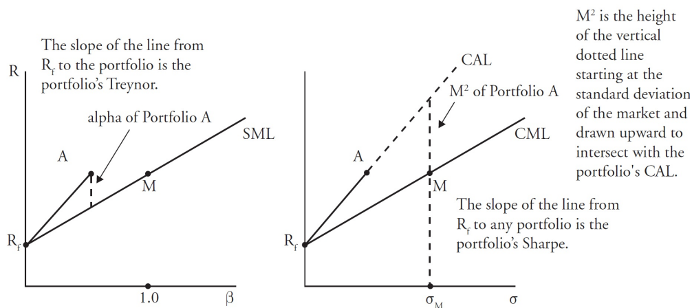
Figure 4: Risk-Adjusted Measures
