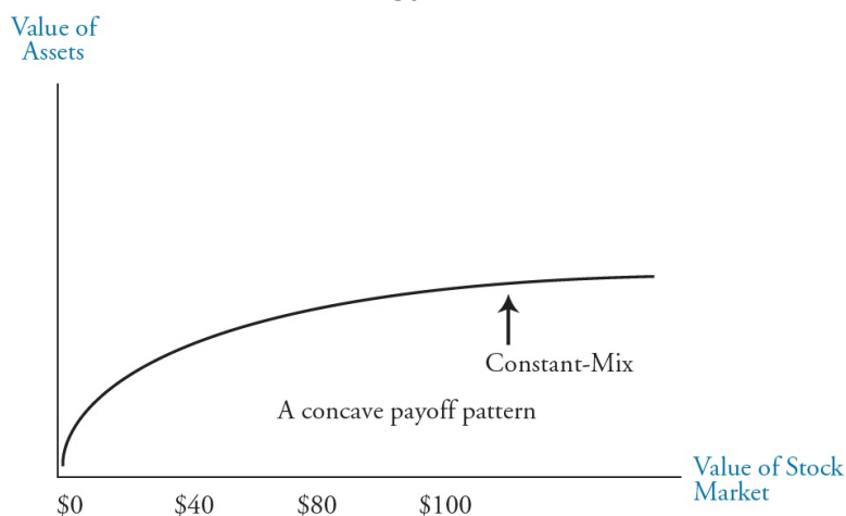
Figure 2: Constant-Mix Strategy
