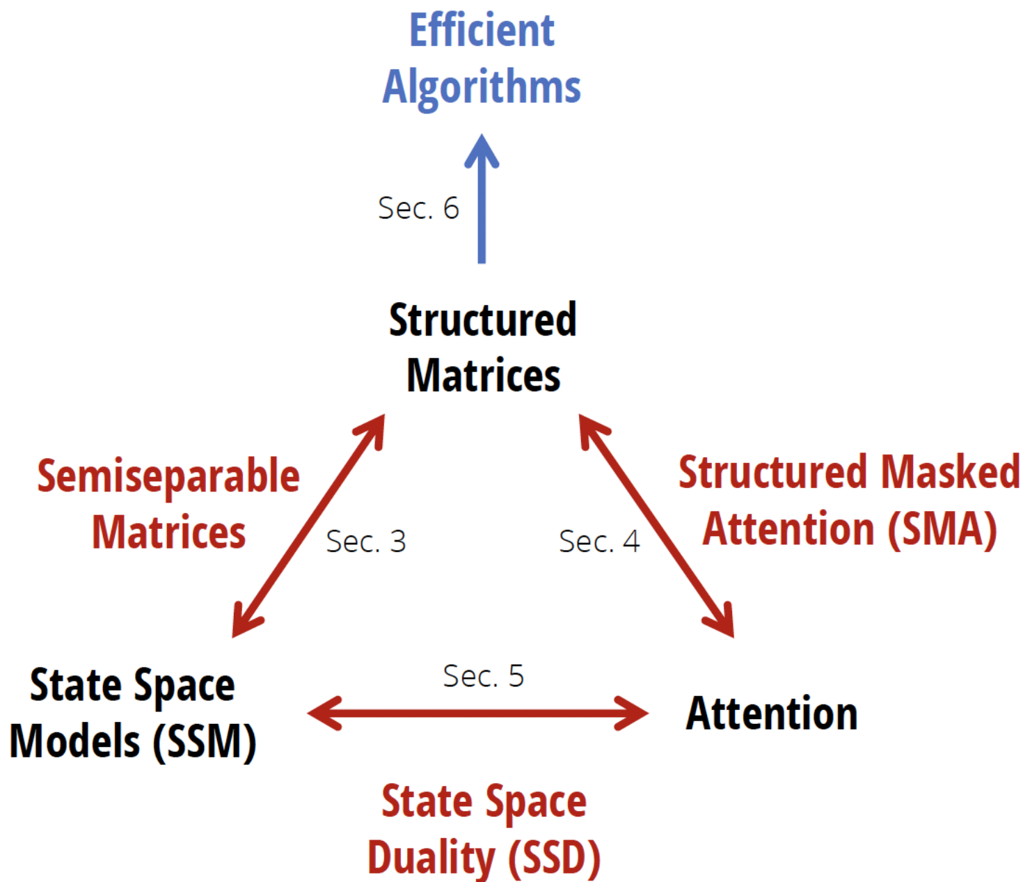
Figure 1: ( Structured State-Space Duality. ) This paper fleshes out the relationship between state space models and attention through the bridge of structured matrices.
