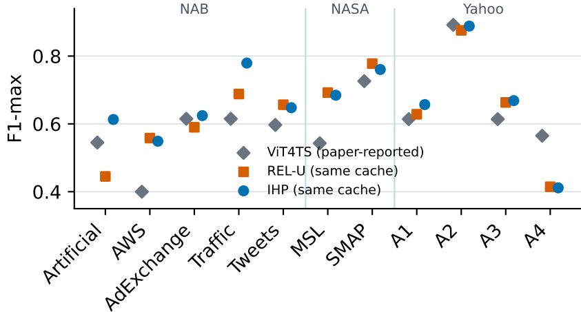
(a) External context and same-cache control
