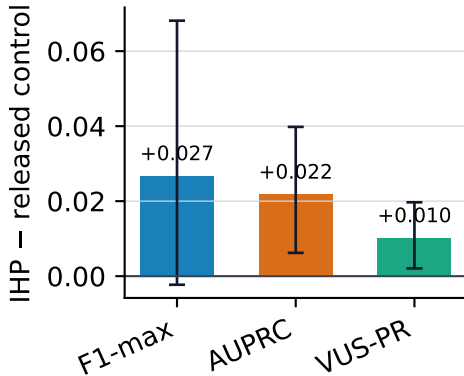
(b) Same-cache ablation
