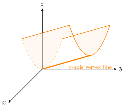
Figure 1.108 The parabolic cylinder z = x^2 .
