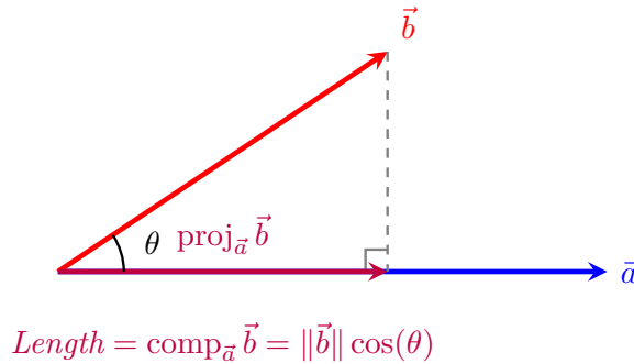
Figure 1.58 The geometric relationship between vector projection and scalar projection.
