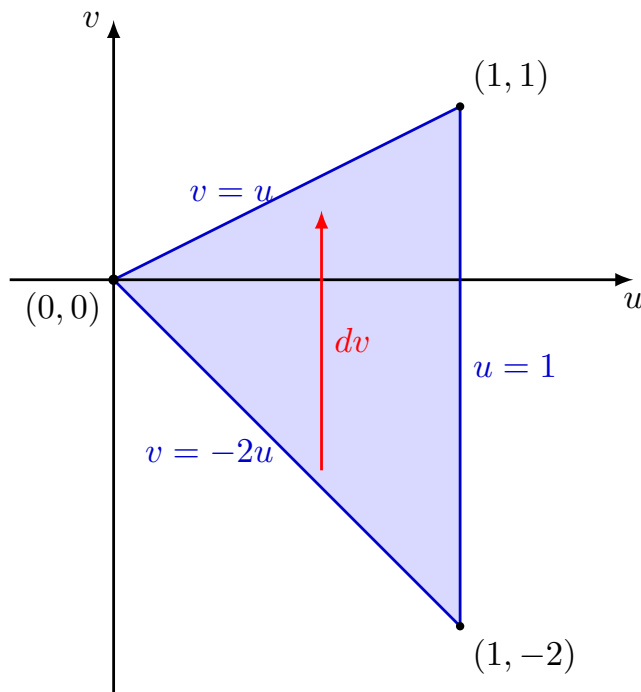
Figure 6.4 The transformed triangular region S inside the uv -plane.
