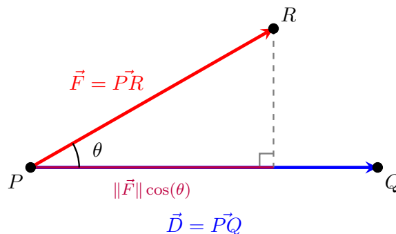
Figure 1.42 The geometric projection of a force vector \vec{F} along a displacement vector \vec{D} .
