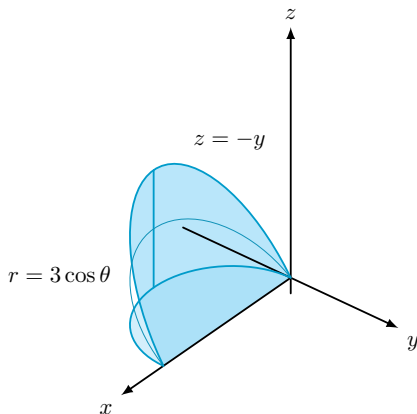
Figure 4.68 The 3D solid wedge cut from the cylinder r = 3 \cos \theta by the plane z = -y .
