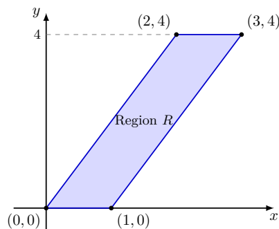
Figure 4.80 The original region R in the xy -plane.
