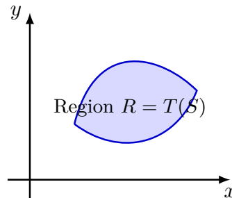
Figure 4.70 The transformed image region R in the xy -plane.
