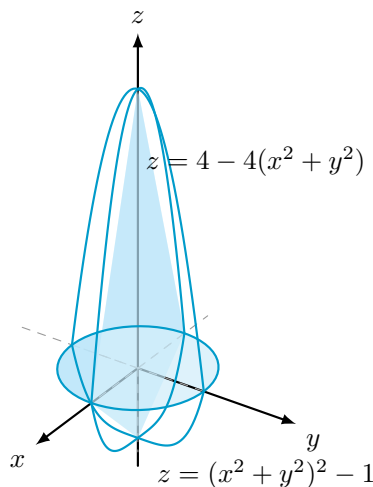
Figure 4.67 3D solid region Q bounded by a paraboloid roof and a quartic floor with fixed shading layers.
