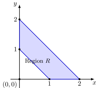
Figure 4.83 The original trapezoidal region R in the xy -plane.
