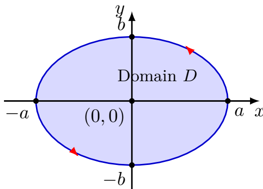
Figure 5.42 The positively oriented boundary curve C enclosing the elliptical region.
