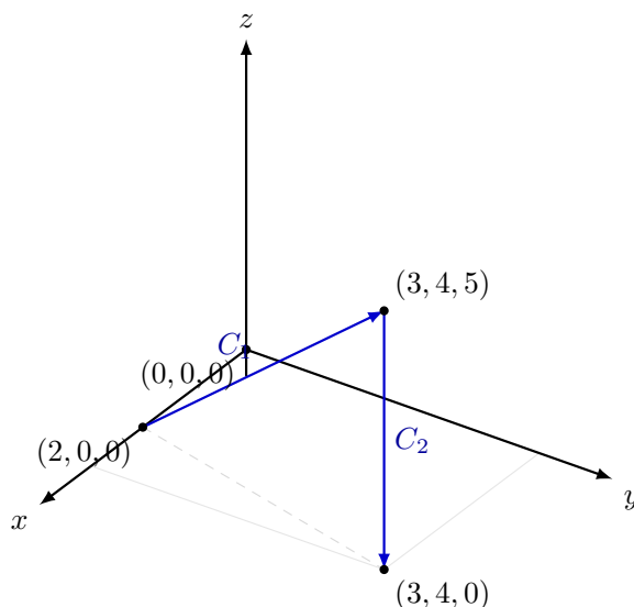
Figure 5.22 The piecewise space path C = C_1 \cup C_2 tracing through three-dimensional space.
