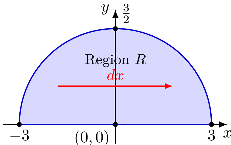
Figure 6.1 The upper half-ellipse region R with horizontal sweeping arrows indicating Type II integration.
