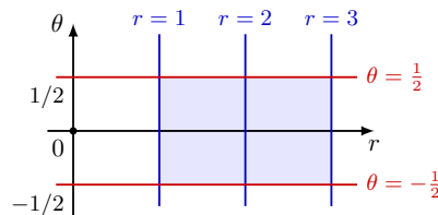
Figure 4.75 Constant grid lines plotted inside the r\theta -plane.
