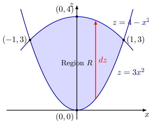
Figure 4.54 The projection footprint region R in the xz -plane bounded by z = 3x^2 and z = 4 - x^2 .
