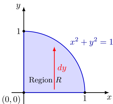
Figure 4.50 The first-quadrant quarter-disk base projection region R plotted with a 1:1 isometric ratio.
