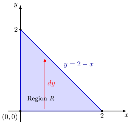
Figure 4.59 The projection footprint region R in the xy -plane bounded by the coordinate axes and the intersection line x + y = 2 .
