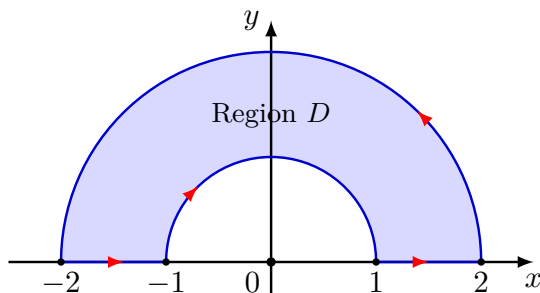
Figure 5.44 The semi-annular integration domain D and its complete closed boundary path C .
