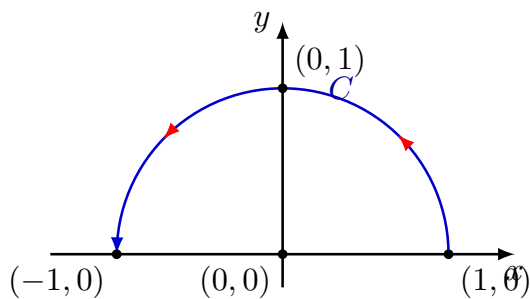
Figure 5.10 The upper semicircular path C plotted with a balanced 1:1 ratio.
