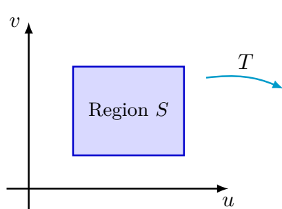
Figure 4.69 The original region S in the uv -plane.
