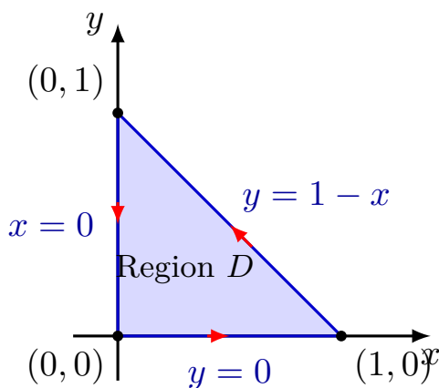
Figure 5.37 The positively oriented closed triangular path C = \partial D enclosing region D .
