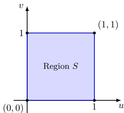
Figure 4.72 The square domain region S in the uv -plane.
