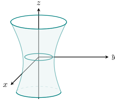
Figure 1.114 A hyperboloid of one sheet.
