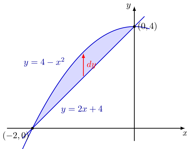
Figure 6.2 The integration domain bounded above by the parabola y = 4 - x^2 and below by the line y = 2x + 4 .
