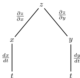
Figure 3.49 Dependency tree diagram for Case I of the Multivariate Chain Rule.
