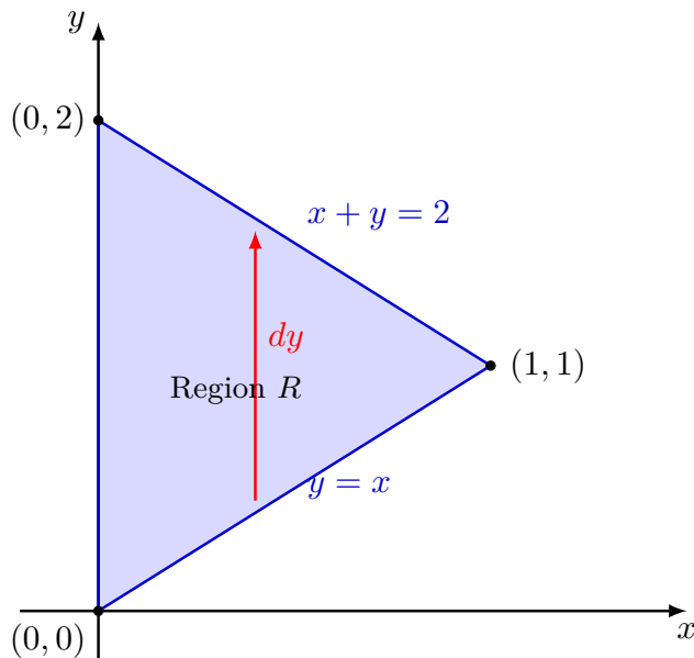
Figure 6.3 The triangular base region R inside the first quadrant with a vertical sweep arrow.
