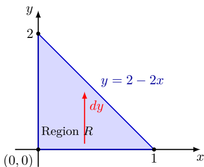
Figure 4.57 The 2D projection footprint R of the tetrahedron in the xy -plane.
