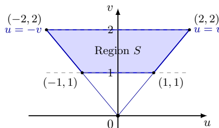
Figure 4.84 The transformed region S in the uv -plane.
