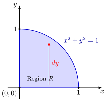
Figure 4.58 The projection footprint region R of the Steinmetz solid in the xy -plane (First Octant).
