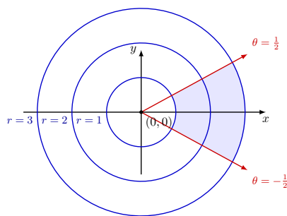
Figure 4.76 The corresponding r -curves and \theta -curves inside the xy -plane.
