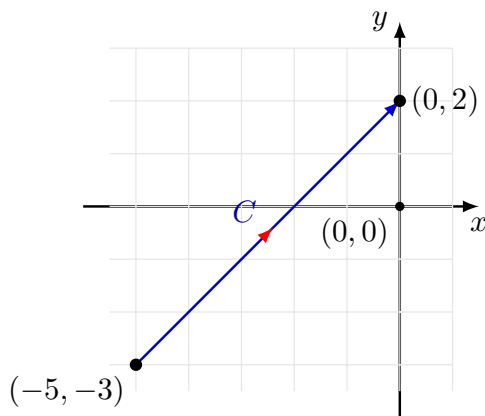
Figure 5.14 The directed straight line segment path C plotted with a balanced 1:1 ratio.
