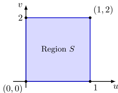
Figure 4.81 The transformed rectangular region S in the uv -plane.
