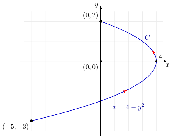
Figure 5.16 The directed parabolic arc path C plotted with a balanced 1:1 ratio.
