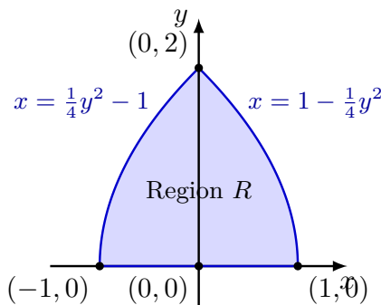
Figure 4.73 The transformed image region R in the xy -plane.
