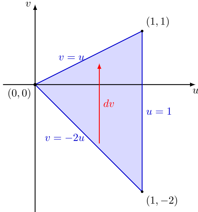
Figure 6.4 The transformed triangular region S inside the uv -plane.
