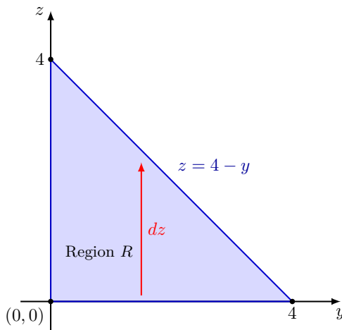
Figure 4.56 The projection footprint region R in the yz -plane bounded by z = 0 , y = 0 , and the line z = 4 - y .
