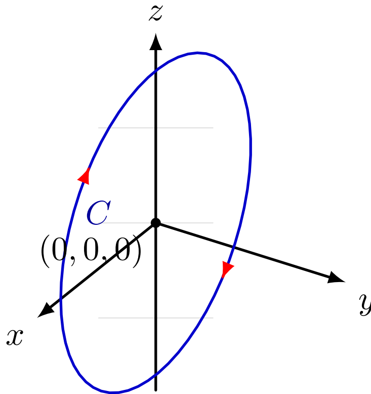
Figure 6.5 The circular integration path C lying entirely within the vertical xz -plane.
