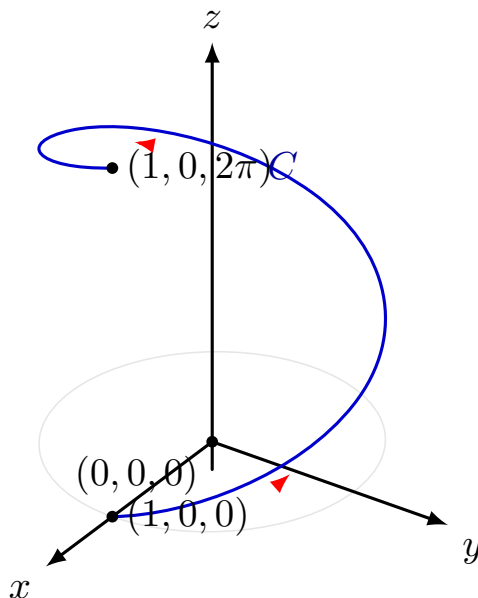
Figure 5.20 The circular helix path C tracing smoothly upward in 3D space from t = 0 to t = 2\pi .
