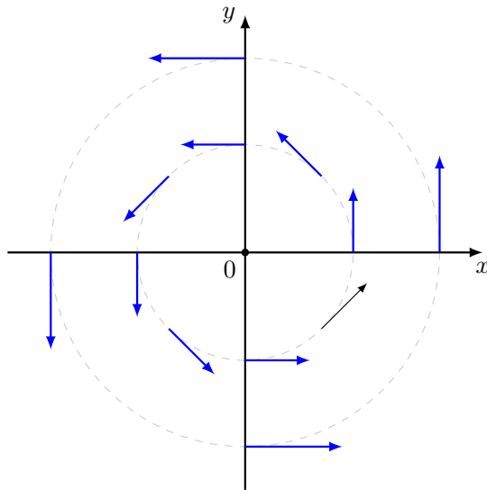
Figure 5.4 Sample vectors from the field \mathbf{F}(x, y) = \langle -y, x \rangle indicating a counterclockwise rotation.
