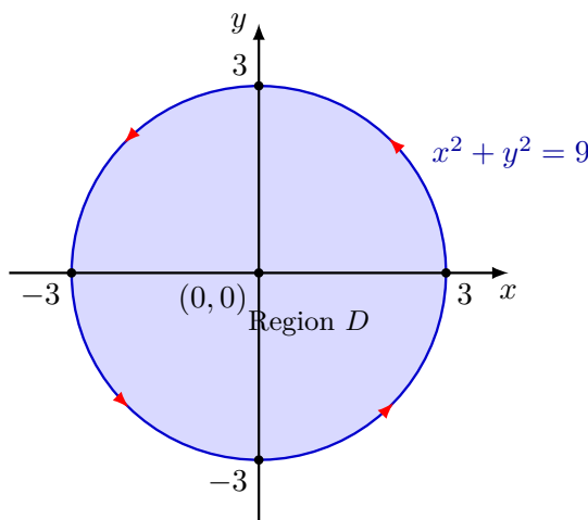
Figure 5.39 The positively oriented boundary circle C : x^2 + y^2 = 9 enclosing region D .
