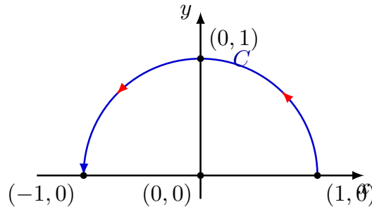
Figure 5.10 The upper semicircular path C plotted with a balanced 1:1 ratio.
