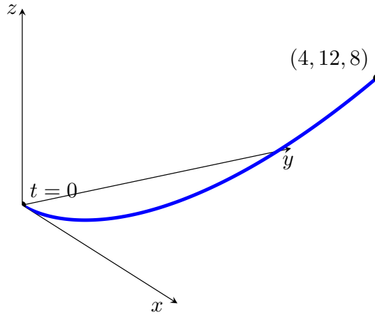
Figure 2.65 The 3D space trajectory of the particle from t = 0 to t = 2 .
