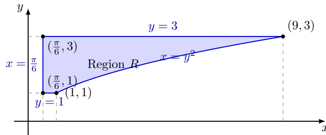
Figure 4.9 The region R : \pi/6 \leq x \leq y^2, 1 \leq y \leq 3 in the xy -plane.
