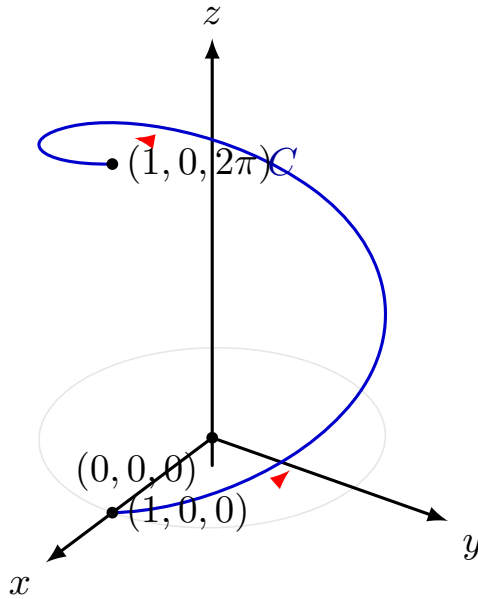
Figure 5.20 The circular helix path C tracing smoothly upward in 3D space from t = 0 to t = 2\pi .
