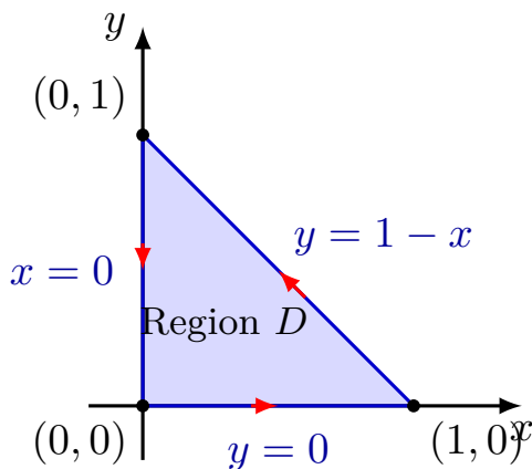
Figure 5.37 The positively oriented closed triangular path C = \partial D enclosing region D .
