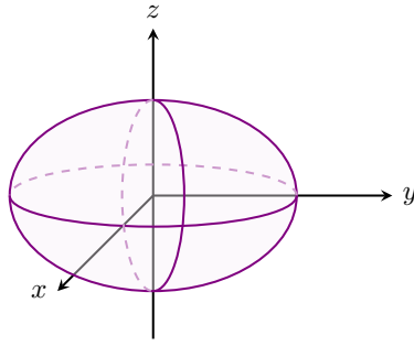
Figure 1.113 A symmetrical ellipsoid centered at the origin.
