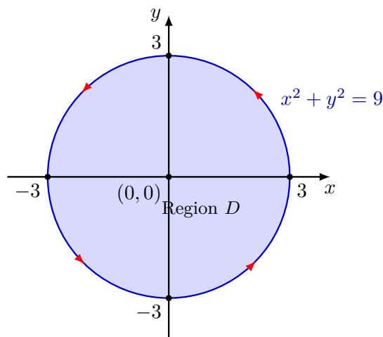
Figure 5.39 The positively oriented boundary circle C : x^2 + y^2 = 9 enclosing region D .
