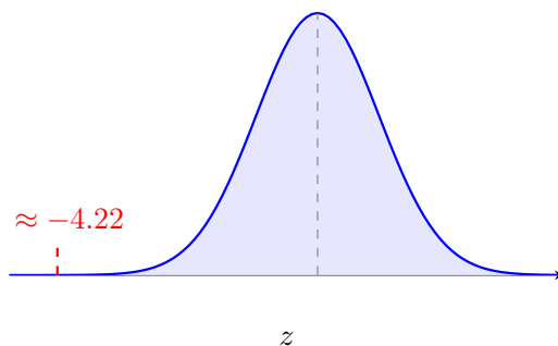
Figure 4.106 Normal distribution curve highlighting an extreme z-score of -4.22.
