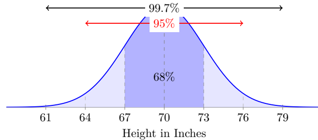
Figure 4.103 Normal Distribution of Heights with Empirical Rule Break-downs
