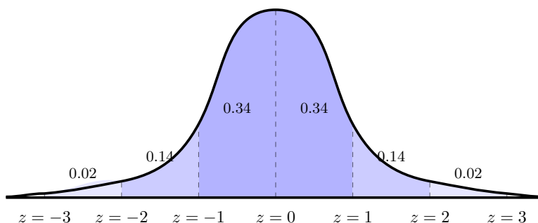
Figure 4.87 The 2-14-34 Rule Area Distribution under a Standard Normal Curve
