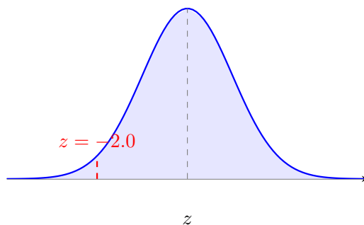
Figure 4.104 Normal distribution curve highlighting a z-score of -2.0.
