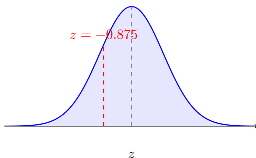
Figure 4.107 Normal distribution curve highlighting a z-score of -0.875.
