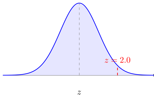
Figure 4.105 Normal distribution curve highlighting a z-score of 2.0.
