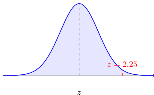
Figure 4.108 Normal distribution curve highlighting a z-score of 2.25.
