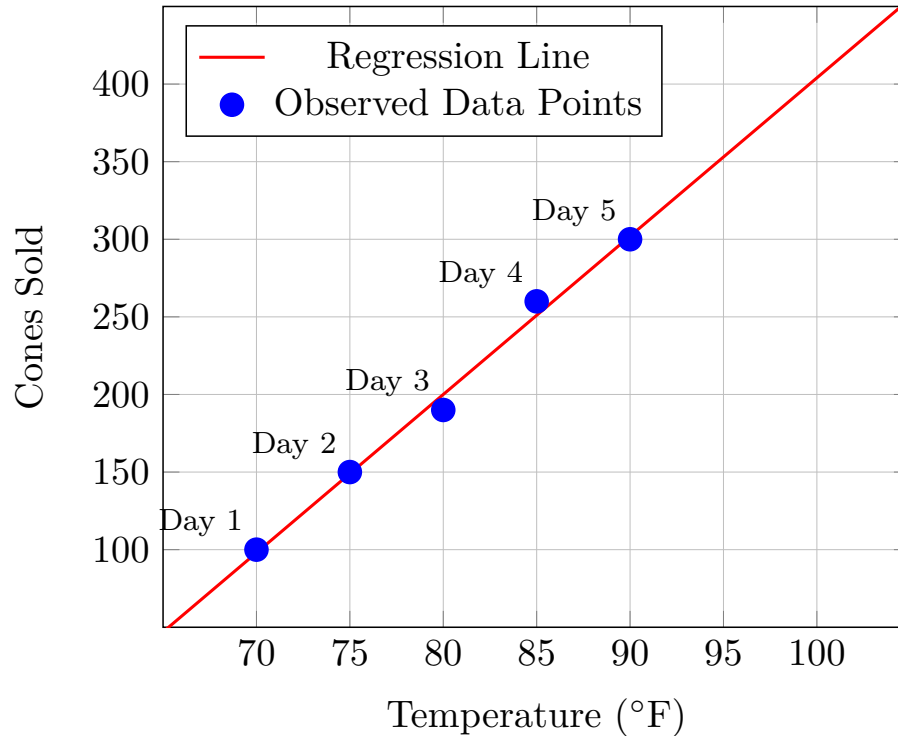
Figure 4.100 Scatter Plot of Temperature vs. Ice Cream Cones Sold
