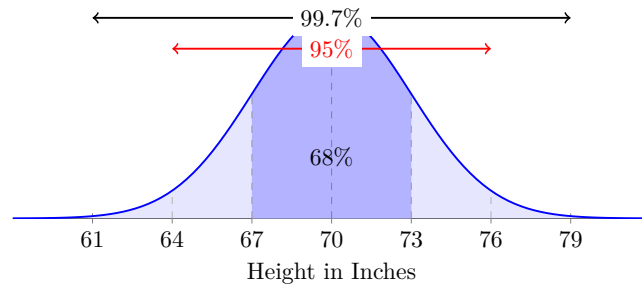
Figure 4.120 Normal Distribution of Heights with Empirical Rule Break-downs
