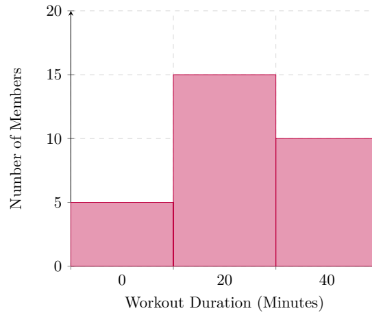
Figure 4.18 Frequency distribution across adjacent numerical bins.
