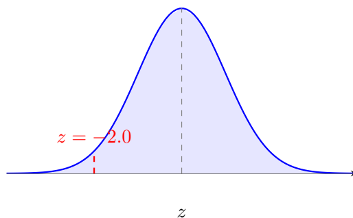
Figure 4.121 Normal distribution curve highlighting a z-score of -2.0.
