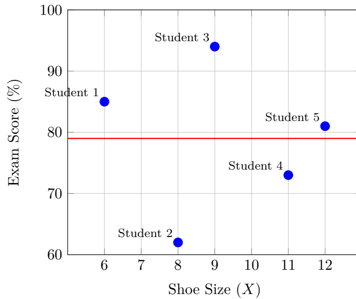
Figure 4.106 Scatter Plot of Shoe Size vs. Exam Score
