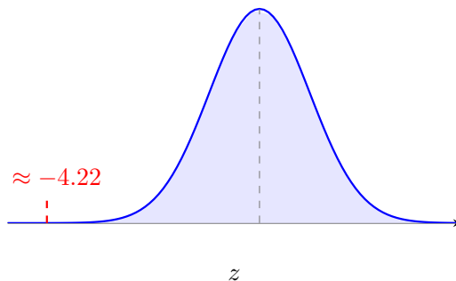
Figure 4.123 Normal distribution curve highlighting an extreme z-score of -4.22.
