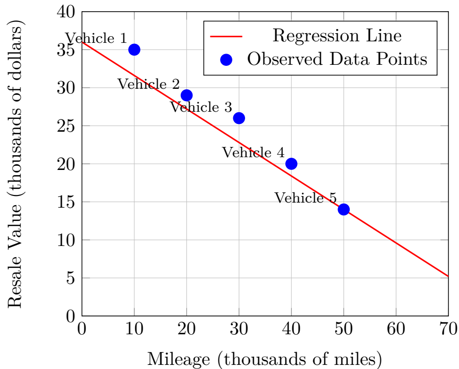
Figure 4.103 Scatter Plot of Mileage vs. Resale Value
