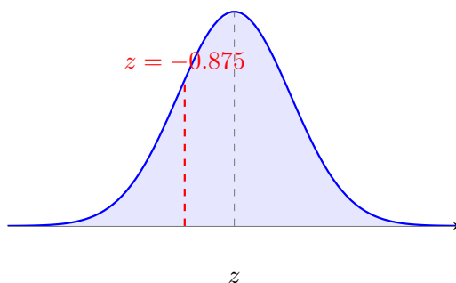
Figure 4.124 Normal distribution curve highlighting a z-score of -0.875.
