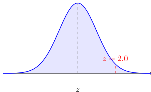
Figure 4.122 Normal distribution curve highlighting a z-score of 2.0.
