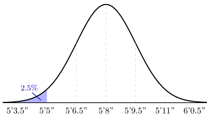
Figure 4.127 Normal distribution curve of women's heights with the lower tail below 5' 5" shaded.
