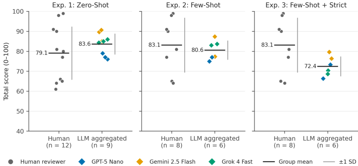
Figure 1. Total score distributions by experiment. Circles show individual human review scores. Diamonds show iteration-averaged LLM scores by vendor (three iterations averaged within each vendor-application combination). Horizontal bars indicate group means (annotated). Vertical bars \pm 1 indicate standard deviation. As shown, LLM scores have a substantially narrower range than human scores in all three conditions.
