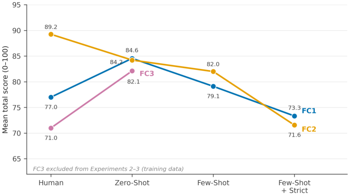
Figure 2. Application-level mean total scores by evaluator condition. Lines connect the same application (FC1, FC2, FC3) across the human panel and the three LLM prompt conditions (LLM values are means of vendor-aggregated scores). Humans separated applications by 18.2 points, whereas zero-shot LLM scores compressed all three applications into a 2.4-point range. Human rank ordering (FC2 > FC1) was reproduced only in the few-shot condition. FC3 is absent from Experiments 2–3, in which it served as training data.
