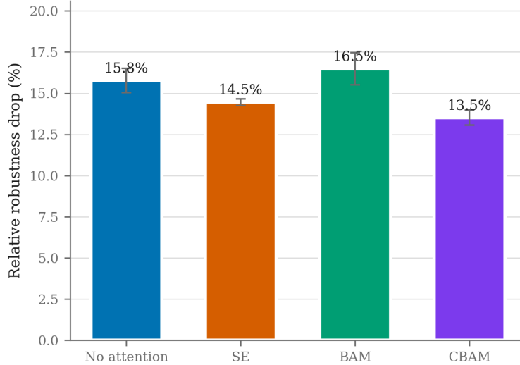
Figure 5: Relative robustness drop, (\text{clean} - \text{corrupted})/\text{clean} , per arm with across-seed standard deviation. Normalising by each arm’s own clean accuracy prevents an arm that starts lower from appearing robust merely because it had less accuracy to lose; the ordering is unchanged from the absolute measure.
