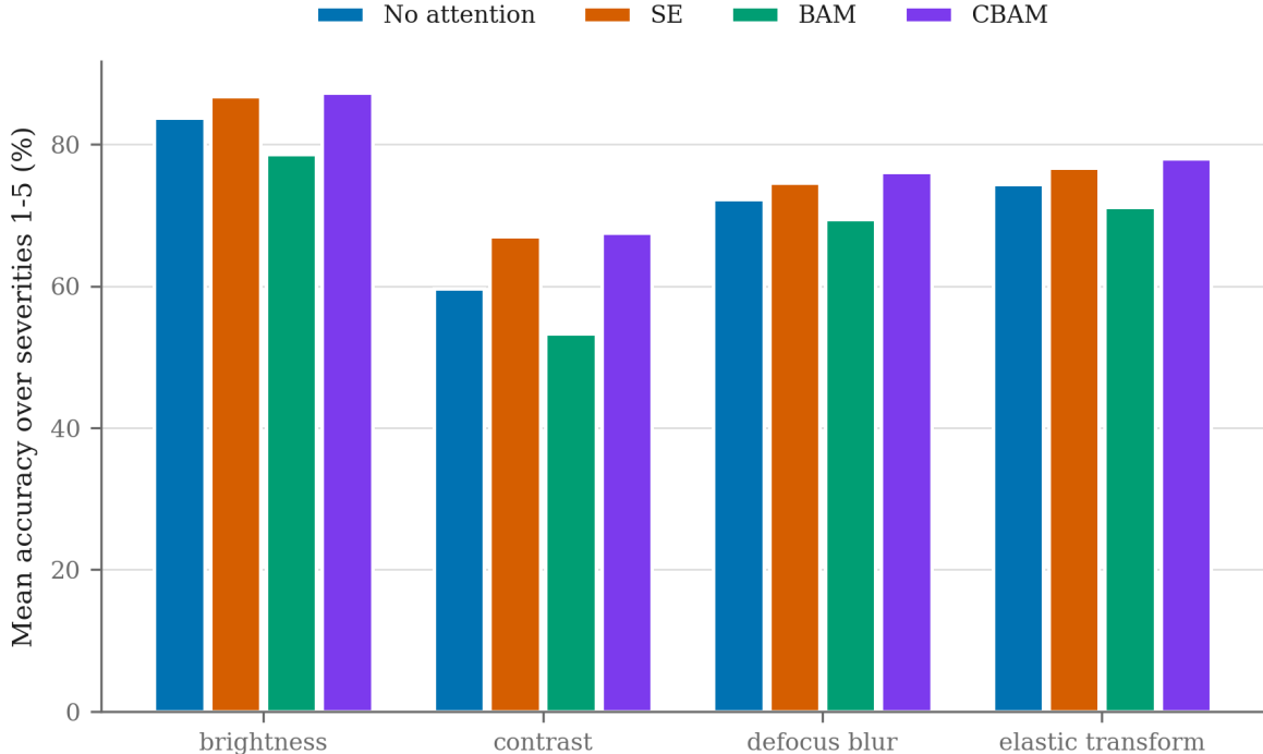
Figure 4: Mean accuracy per corruption type, averaged over severities 1–5 and three seeds. Reporting the breakdown alongside the four-type mean makes a type-specific skew visible: contrast is the most damaging corruption for every arm, and also where the attention arms separate most from the baseline.
