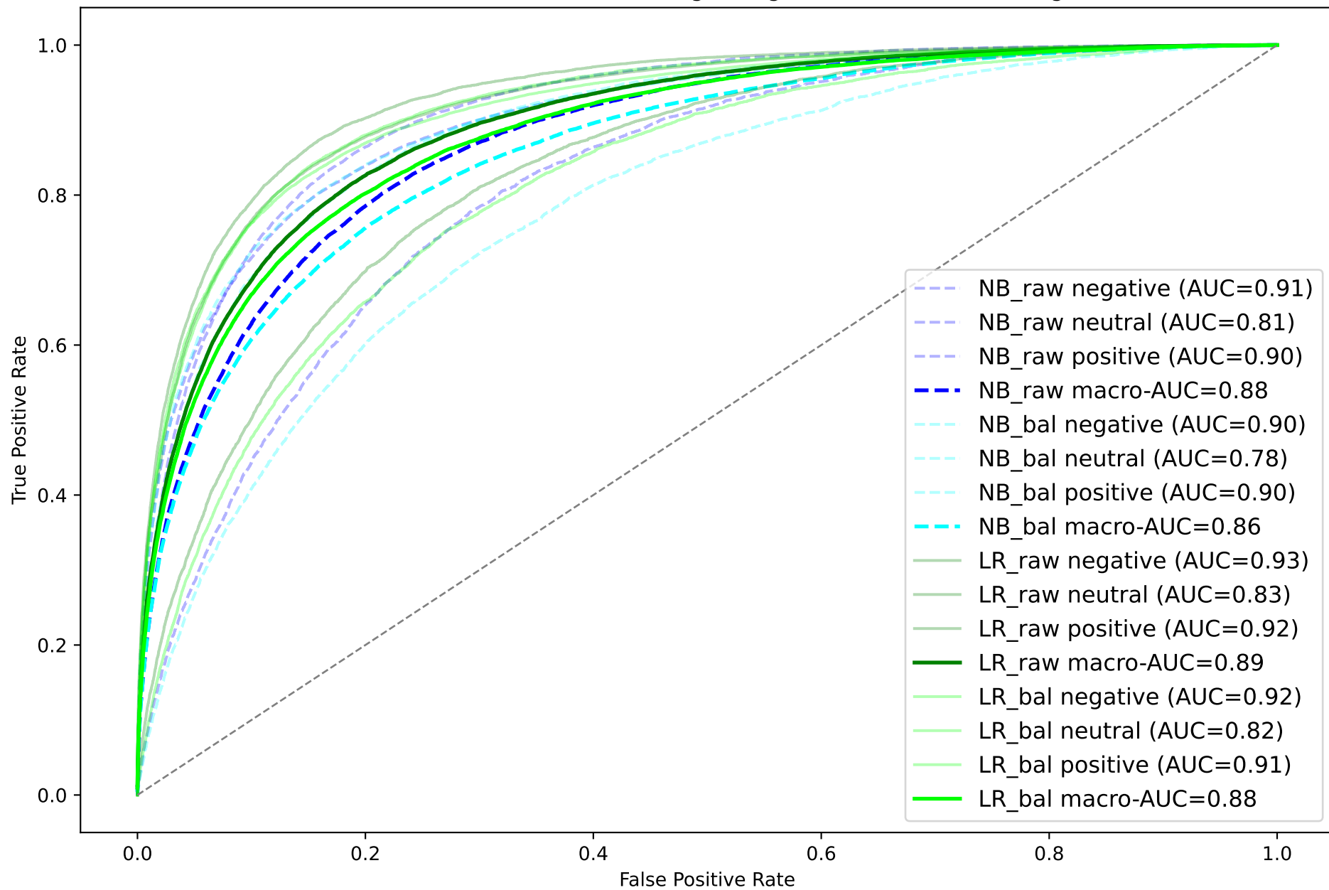
ROC Curves with Macro-Average: Original vs Balanced Training
