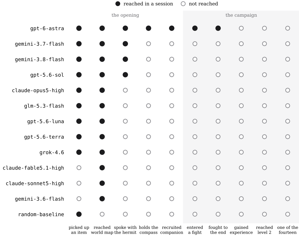
Figure 4: The milestone ladder, one row per model; a filled marker is a rung reached in at least one of its sessions. The evidence behind each rung, and the record it is read from: an item count above its opening count (the bag in memory); the save the game writes on the world map, or the world-map fingerprint of the frame (save, frame); the portrait of the hermit in the dialogue frame (replay); the compass in the bag or its coordinates on the item screen (bag, replay); a party of more than one or the prompt of a companion answered yes (save, replay); the card of the acting character in a fight (replay); the defeat banner or experience gained (replay, record); experience above zero and a level above one (character record); a book in the bag or carried by the protagonist (bag, record).
