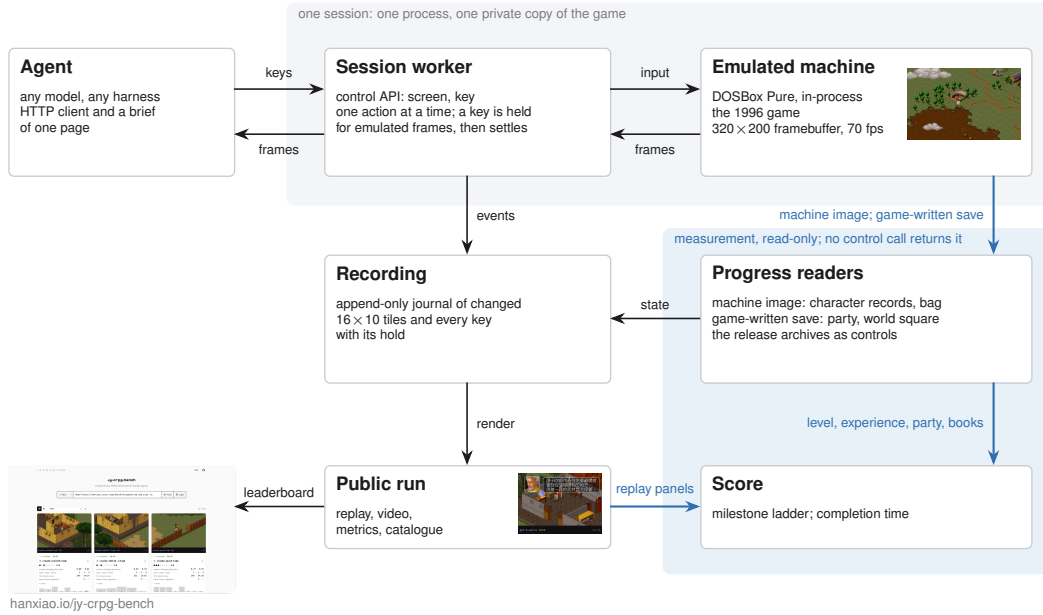
Figure 3: One process per session loads the game core and answers the control API; the recording feeds the public replay, and progress is read from the emulated machine, from the save the game writes and from the replay, on paths no control call reaches.
