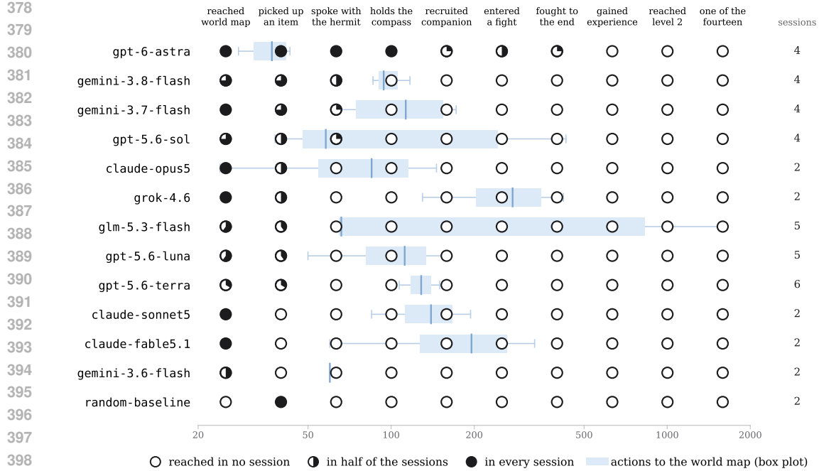
Figure 4: Milestones per model, ordered by milestones reached, then by the shares from the deepest milestone down, then by median actions to the world map. Each marker shows the share of sessions in which the model reached the milestone, and the number of sessions is given at the right. The box plot behind each row shows the actions taken to reach the world map across the sessions that crossed, on a log scale, with the box spanning the quartiles, the line inside it the median, and the thin line the range. The evidence for each milestone, and the record it comes from, is: a save written on the world map, or the world-map fingerprint (save, frame); an item count above the starting count, or the pickup message on screen (memory, replay); the portrait of the hermit (replay); the compass in the bag or on the item screen (memory, replay); a party of more than one, or a yes to the join prompt (save, replay); the card of the acting character (replay); the defeat banner or experience gained (replay, memory); experience above zero and a level above one (memory); a book in the bag or carried by the protagonist (memory). A session with no fight on its replay is counted as having gained no experience and no book, since both require a won fight.
