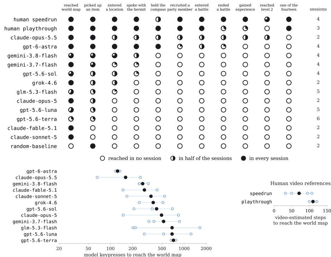
Figure 3: Milestones per model. The upper panel gives the share of sessions in which each model reached each milestone, with the number of sessions at the right; rows are ordered by the milestones reached, with the human references first and the random baseline last. The lower left panel gives the keypresses of each model to the world map on a log scale, with a light dot per session and a black dot for the mean, and the lower right panel the steps of the human references, counted from videos that carry no keyboard log. Appendix D gives the record behind each milestone.
