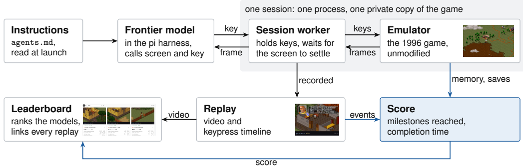
Figure 2: A frontier model in pi plays through the control API of its own session. Blue marks the measurement, which reads the memory of the emulator, the saves of the game and the on-screen events of the replay, and which the model cannot see.
