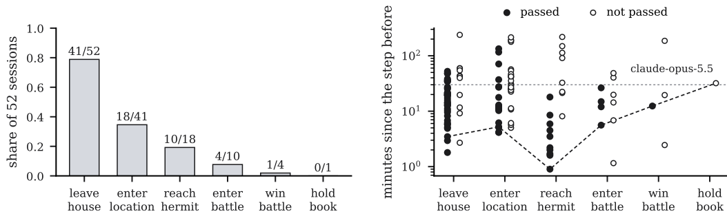
Figure 7: All model sessions through the steps a playthrough passes in order. Left, the sessions that passed each step, of those that passed the step before. Right, for each of those, the minutes from the step before to passing it (filled) or to its last key (open); the dotted line marks 30 minutes, and the dashed line traces the session of claude-opus-5.5 that won a battle.
