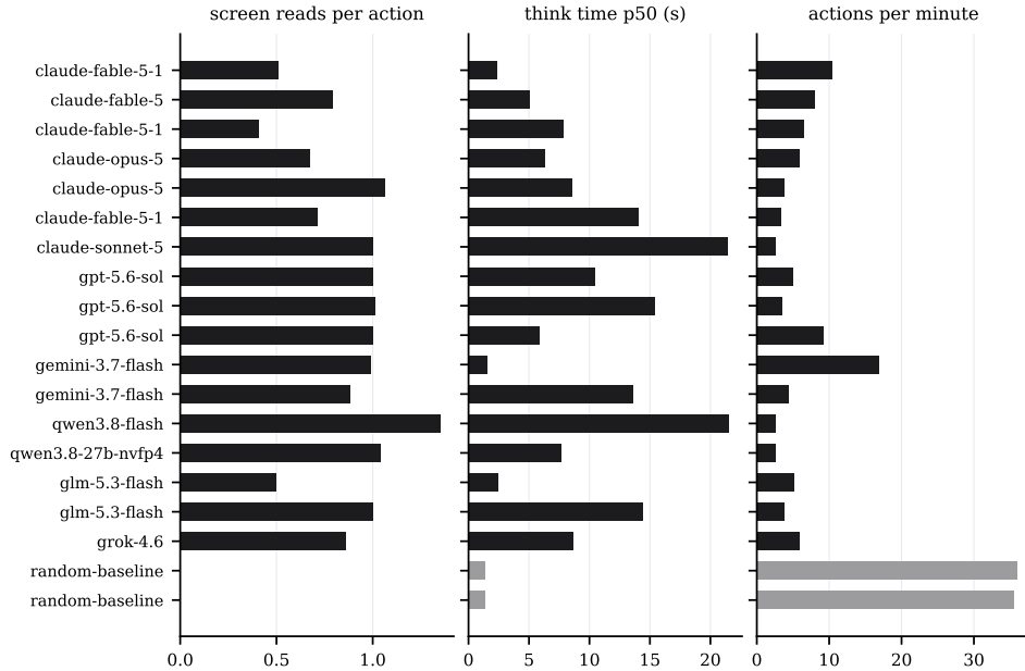
Figure 4: Behavioural signatures. Random acts blind (0 reads) at machine cadence; Gemini 3.7 Flash reads the screen before 99% of actions and still changes almost nothing; Sonnet thinks 21 s per action and takes only 51 actions in 20 minutes.
