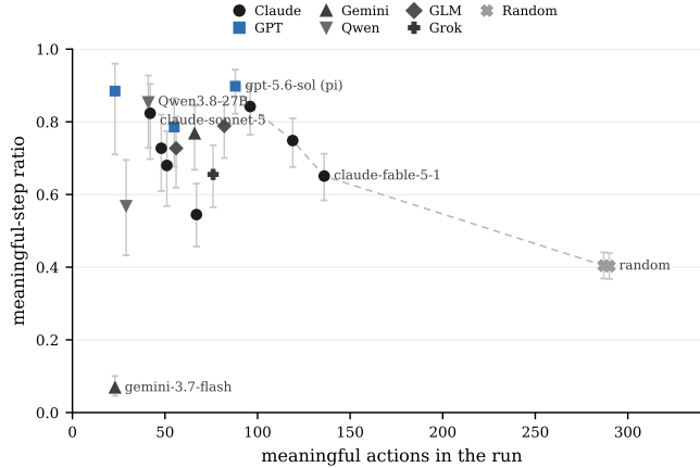
Figure 3: Quality (meaningful-step ratio, with 95% Wilson CIs) against throughput (meaningful actions). Neither axis alone is a score: ratio rewards near-inaction (Qwen: 41 meaningful actions at .854), count rewards mashing (random: 290 at .403). The dashed line is the set of runs dominated by nobody on both axes.
