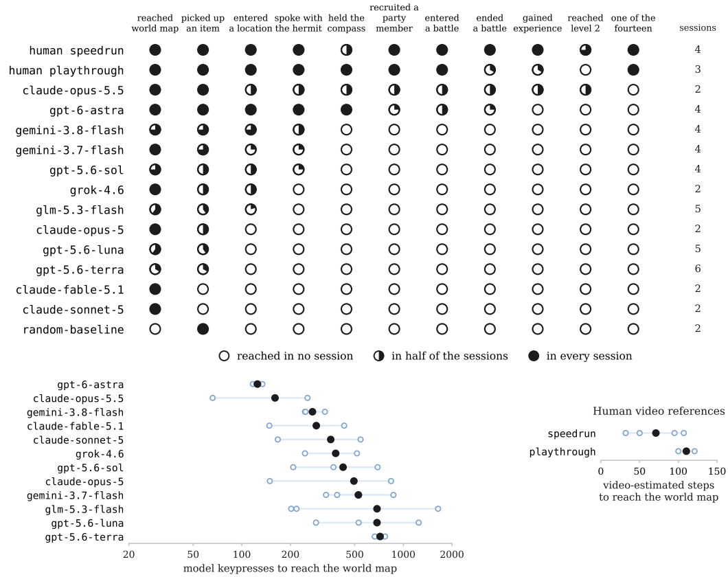
Figure 3: Top, the share of sessions reaching each milestone, ordered by milestones reached, with human references first and the random baseline last. Bottom left, model keypresses to the world map, log-scaled and ordered by their mean. Bottom right, human video-estimated steps on a separate linear axis, not comparable to keypresses. Light dots denote records; black dots their means. Appendix D defines the measures.
