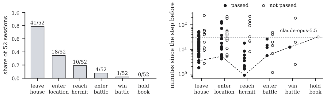
Figure 7: All model sessions through the steps a playthrough passes in order. Left, the bar heights and labels give the share of all 52 sessions that passed each step. Right, among sessions that passed the preceding step, the minutes from that step to passing this one (filled) or to the last key (open); the dotted line marks 30 minutes, and the dashed line traces the session of claude-opus-5.5 that won a battle.
