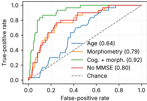
Sparse severity ROC curves
