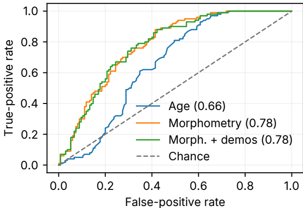
Nonzero CDR ROC curves
