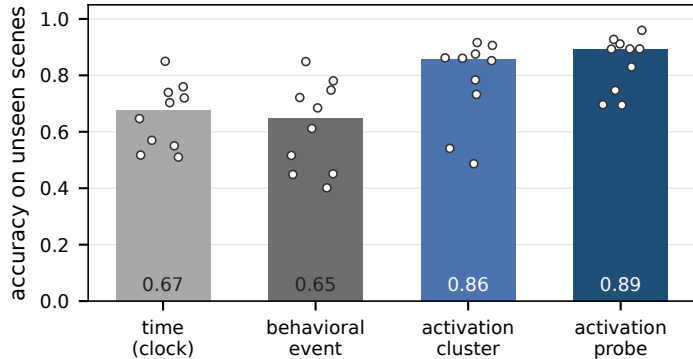
(a) phase readout on unseen scenes: internal vs external
