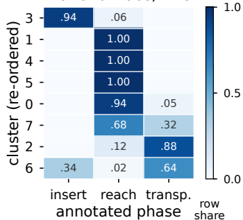
(a) Cluster-phase contingency Pick and Place, k=8
