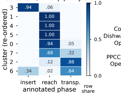
(a) Cluster-phase contingency PPCC candle, k=8 | purity 0.888
