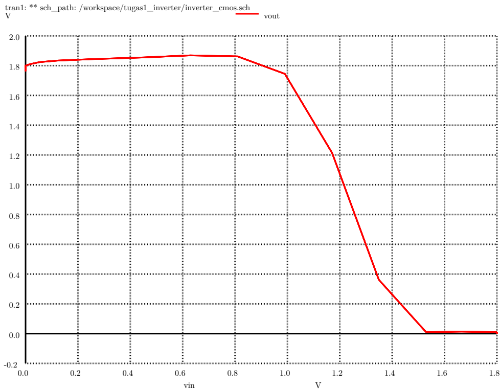
Gambar 3: Karakteristik transfer tegangan DC (VTC).
