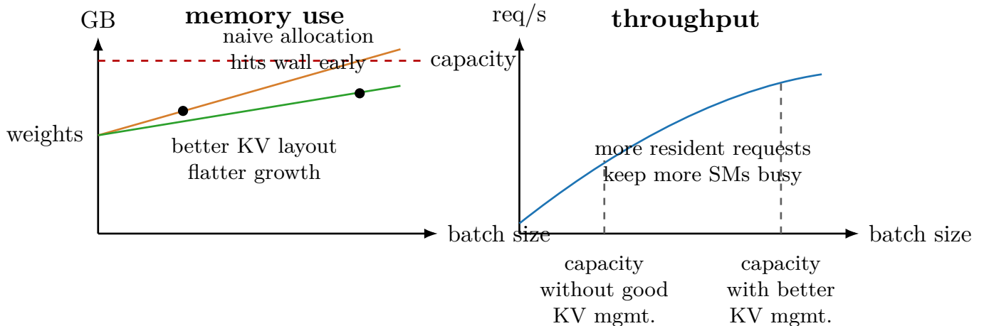
Figure 8: KV-cache management links memory capacity to throughput. If cache allocation grows too fast with batch size, the server hits the memory wall before the GPU reaches its useful throughput region.
