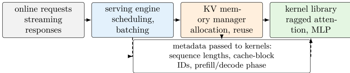
Figure 6: Modern serving stacks split responsibilities. The scheduler decides which requests run; the memory manager decides where KV entries live; optimized kernel libraries execute token-wise and ragged attention work using the metadata supplied by the engine.
