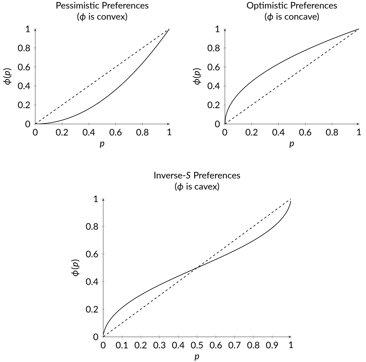
Figure 3: Pessimistic, Optimistic, and Inverse-S Attitudes towards Uncertainty.
