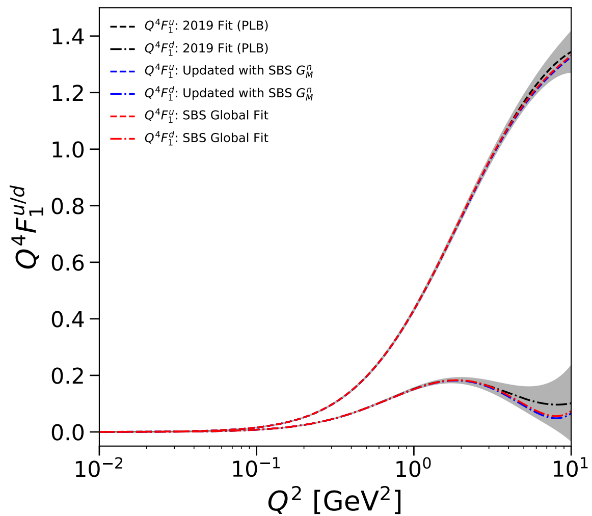
All Sets
