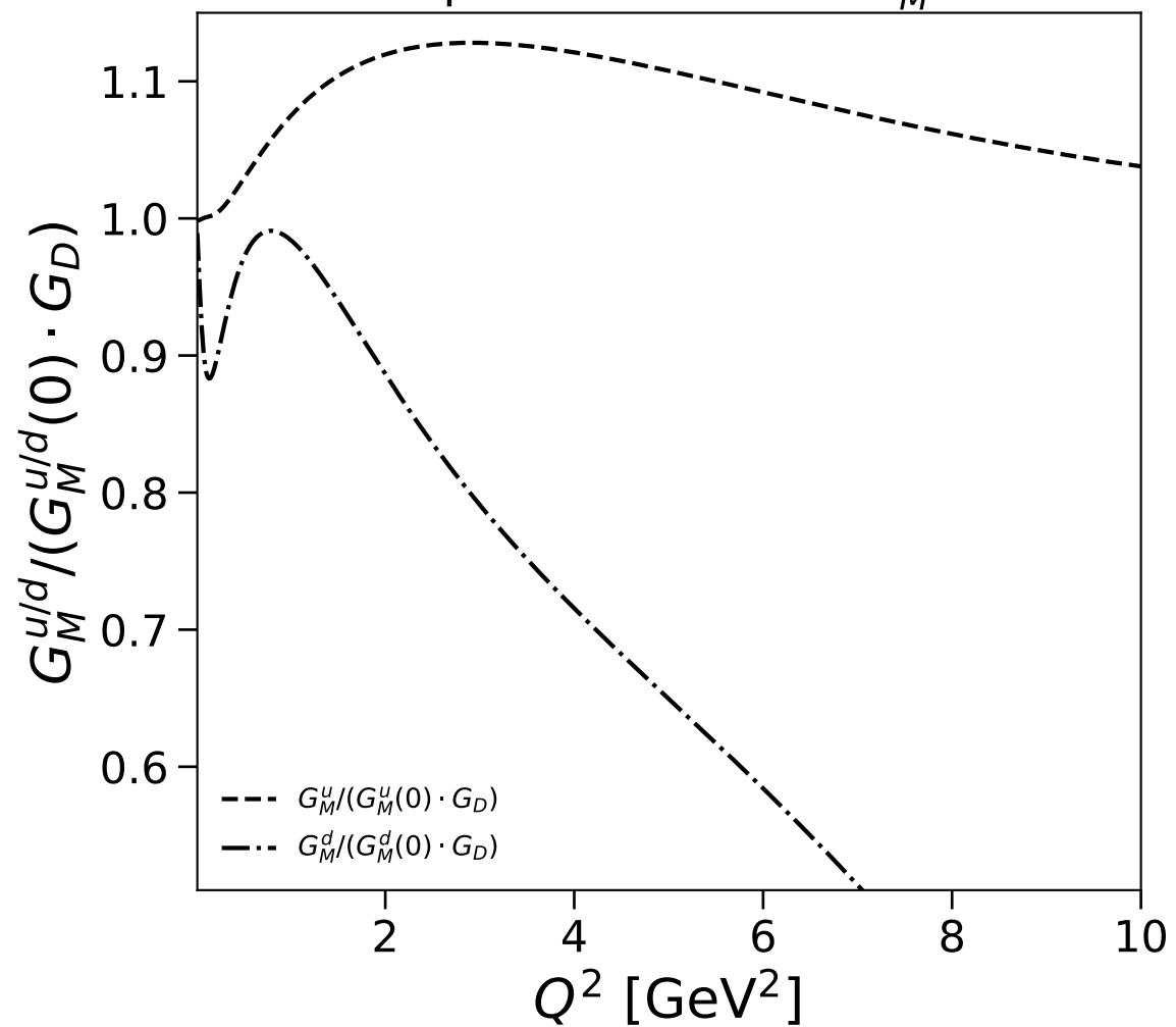
All Sets
