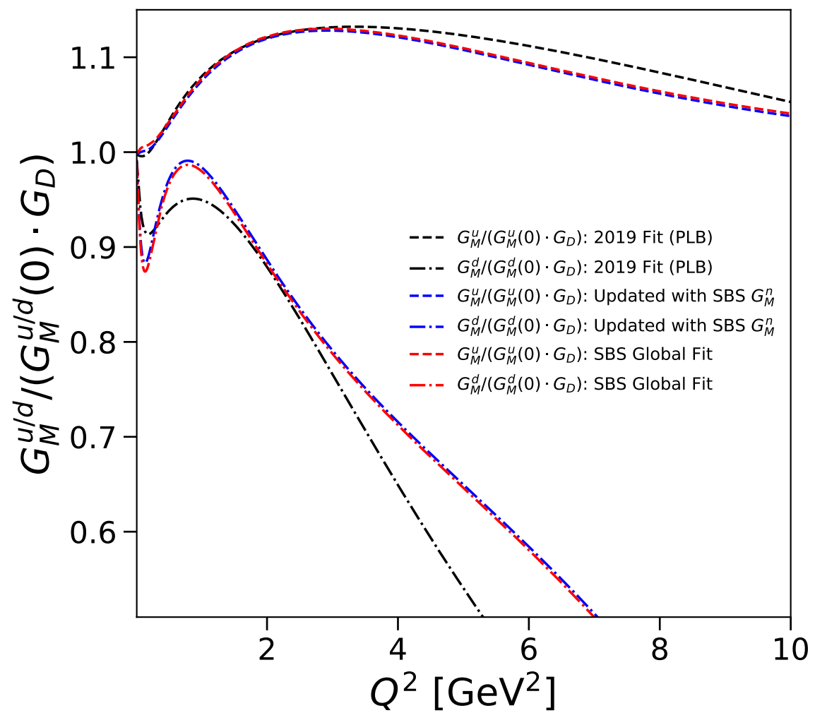
All Sets
